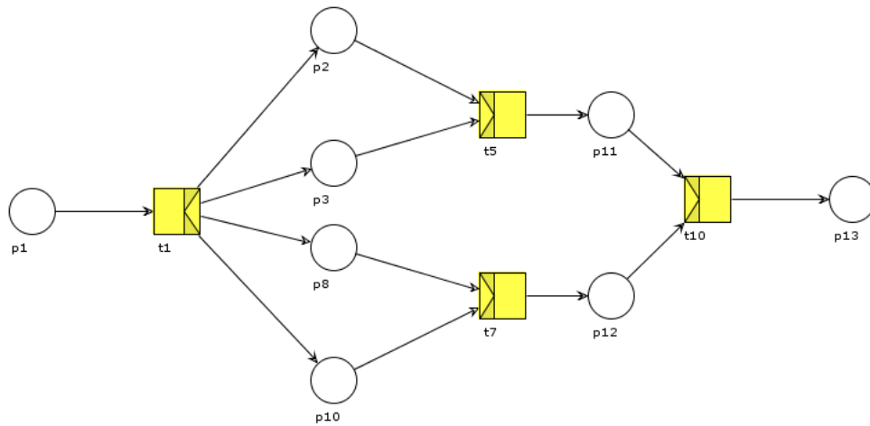
Figure 3: Handle clustering example
