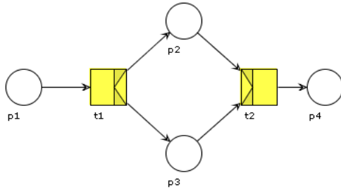
Figure 1: Simple coloring example
